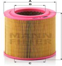
Air Filters C 1430 EM-30171
