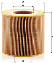
Air Filters C 1381 EM-30197
